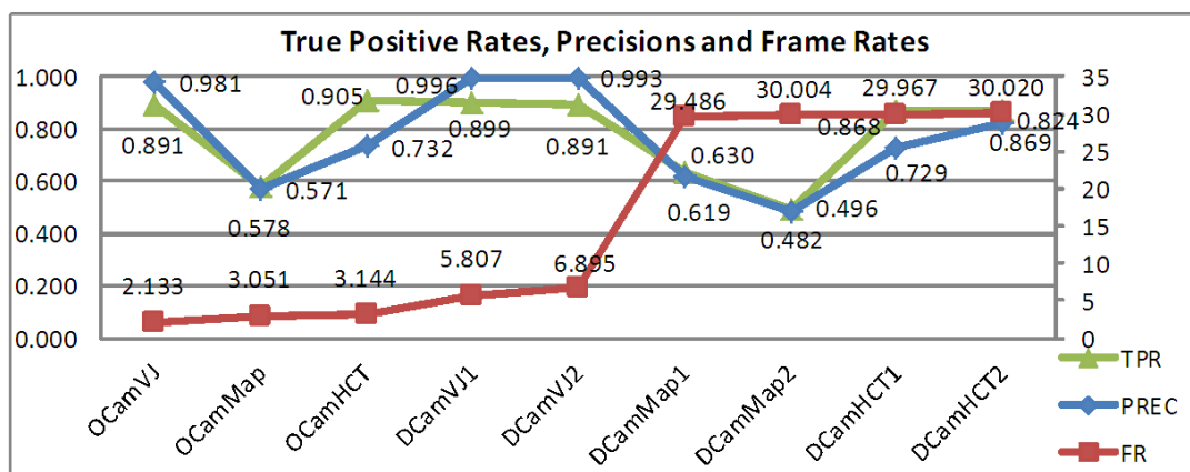
FIGURE 7. Comparisons of true positive rates, precisions, and frame rates
